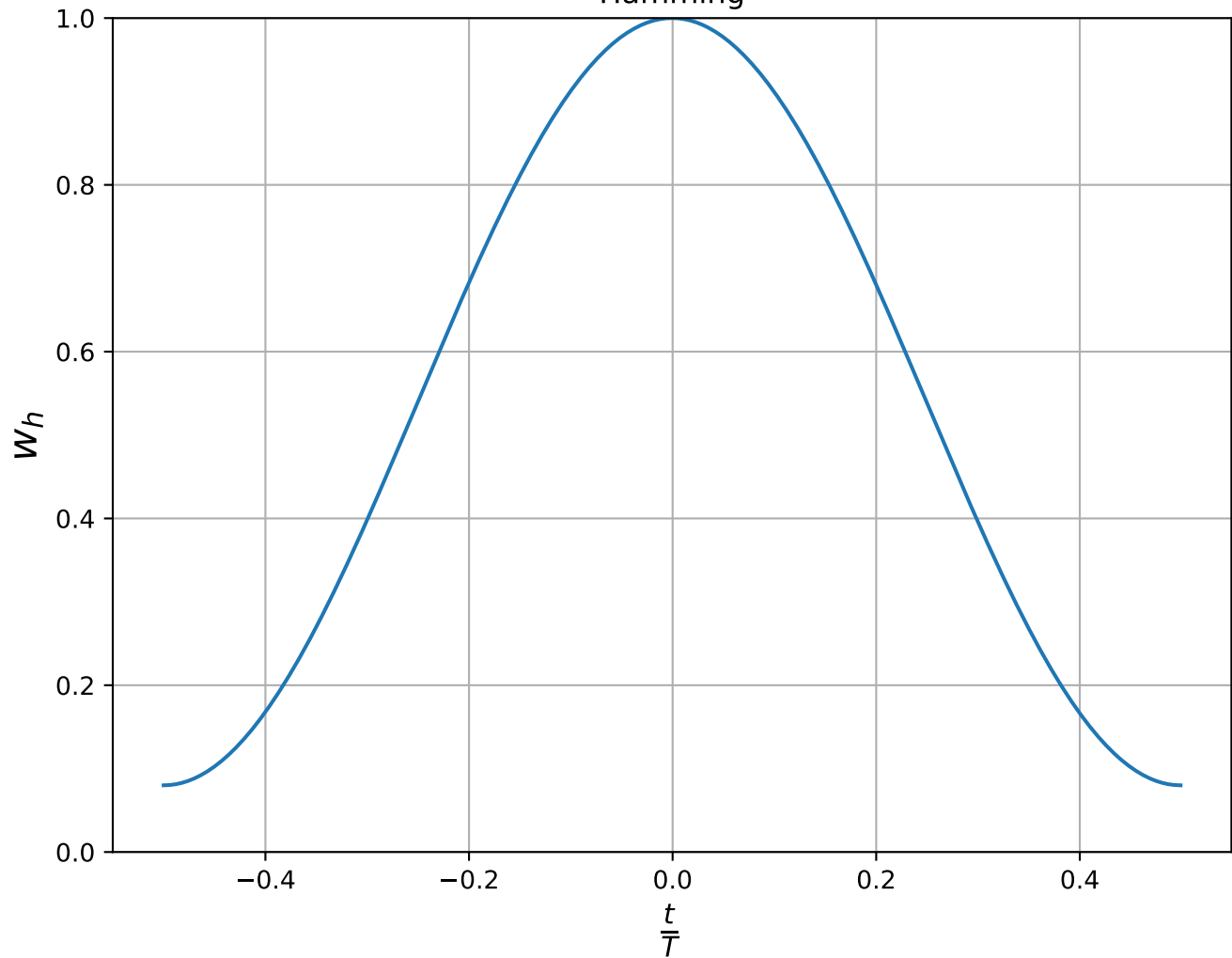
Hamming
