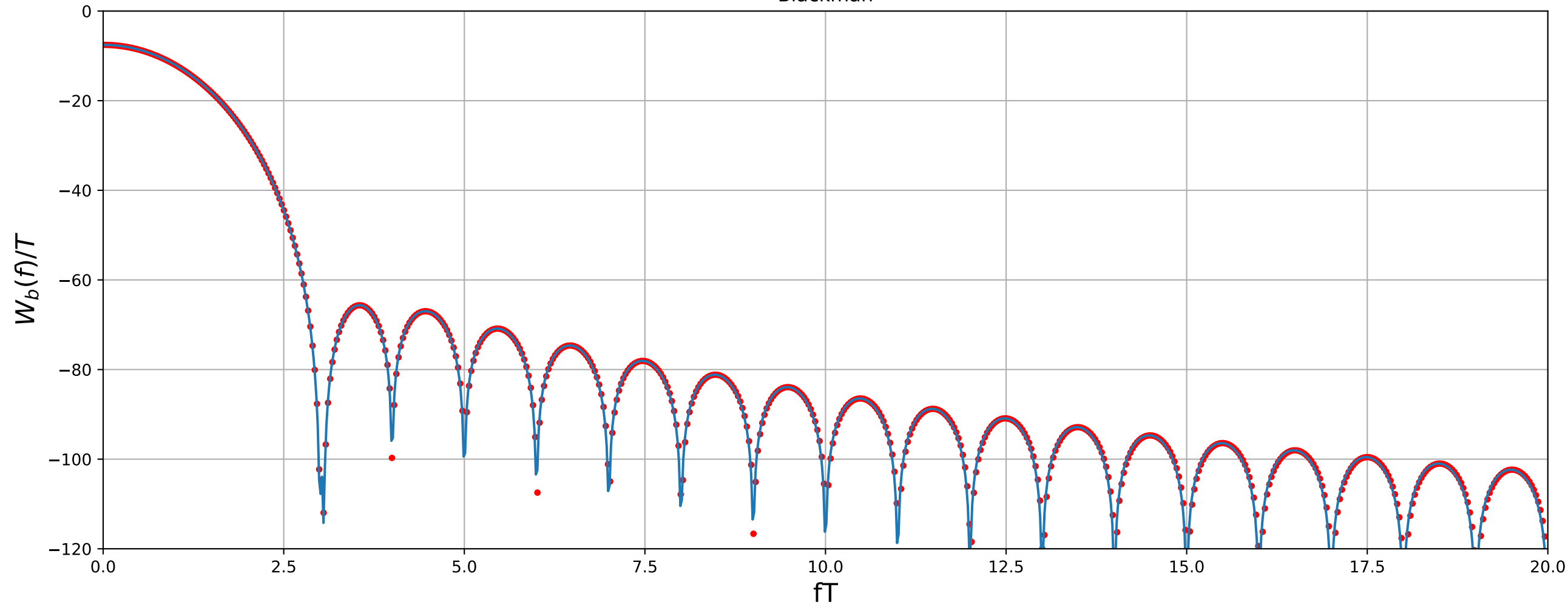
Blackman
